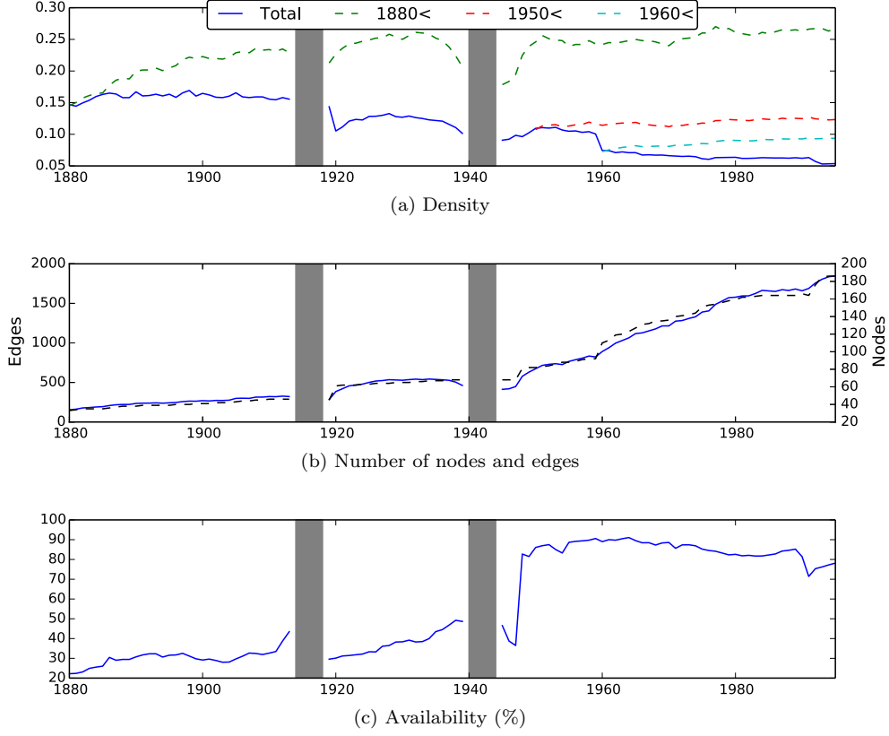
Figure 3: Network density (panel a), number of nodes and edges (panel b) and the availability of the hti (panel c) over time.
